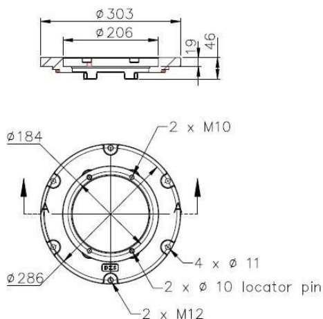
Order Code ADAPTOR 12-8 - 12" Mounting Ring Line Drawing
